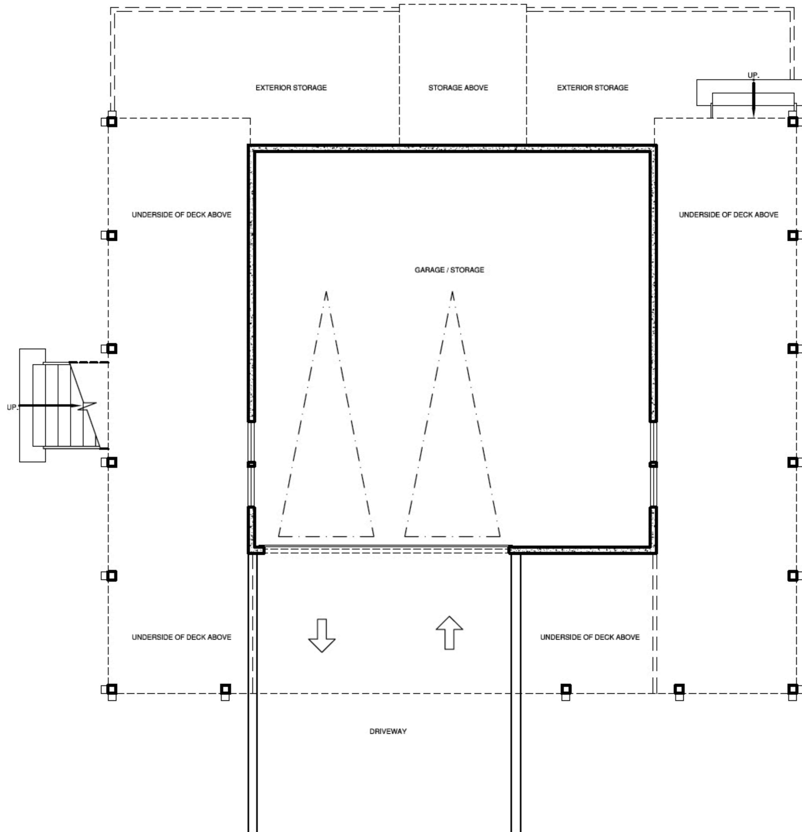
BASEMENT PLAN
